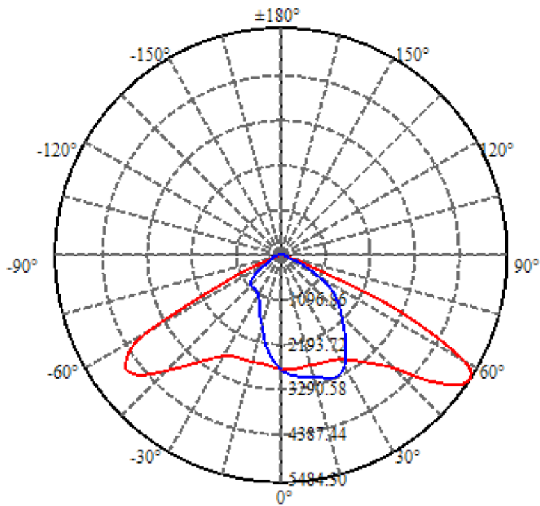
Isocandela diagram
