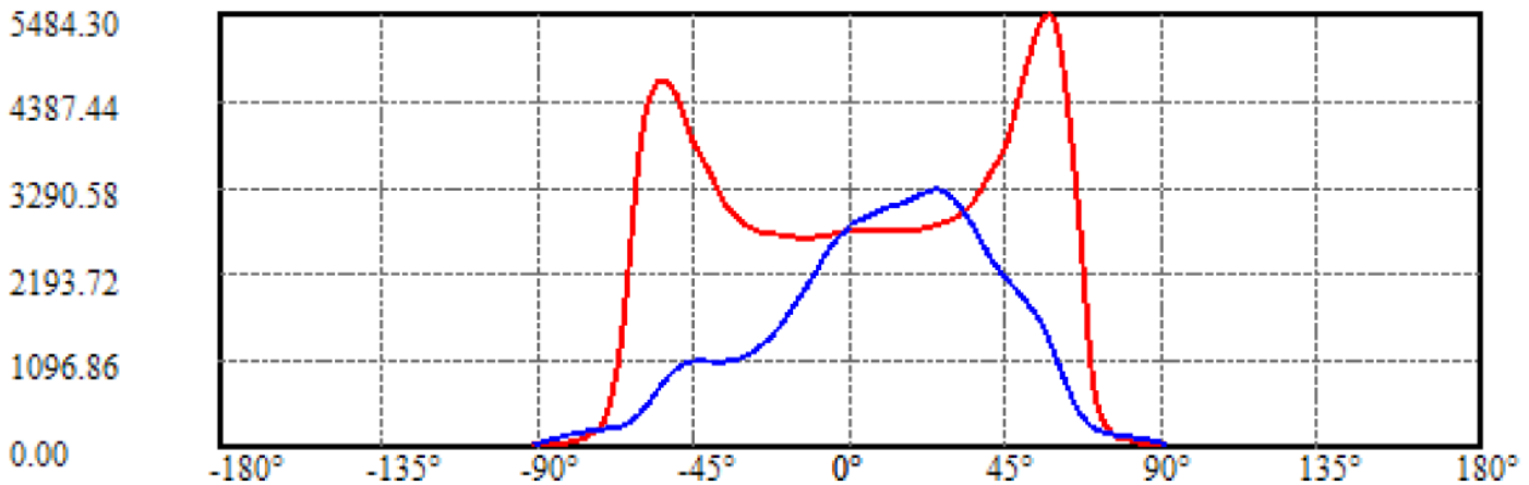
Cartesian coordinates
